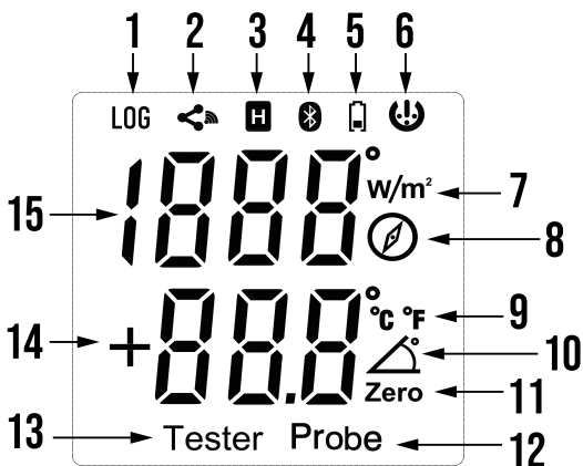
Figure 3.3 Meter display. See descriptions below.
