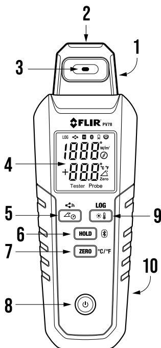
Figure 3.1 Front view of meter. See descriptions below.
