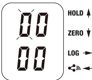
Figure 9.1 Time Stamp setting screen. Upper digits represent hours; lower digits represent minutes. The flashing digit is ready to be adjusted. Use the HOLD and ZERO buttons to change a digit value, and use the LOG and Transmit buttons to step right and left.
