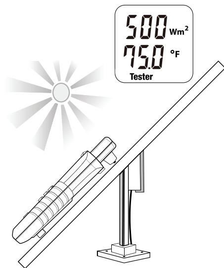
Figure 6.1 Surface temperature measurements using the embedded temperature sensor.
