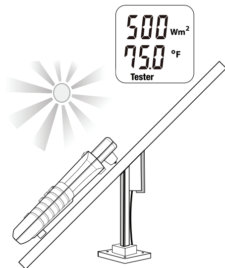
Figure 5.1 Irradiance measurements.
