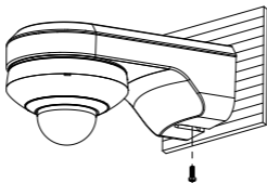
Figure 2-12 Fix the Bracket
